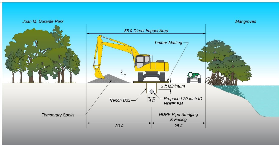
Figure 3-15 Typical Construction Section West Intertidal Zone (Segment 1)
