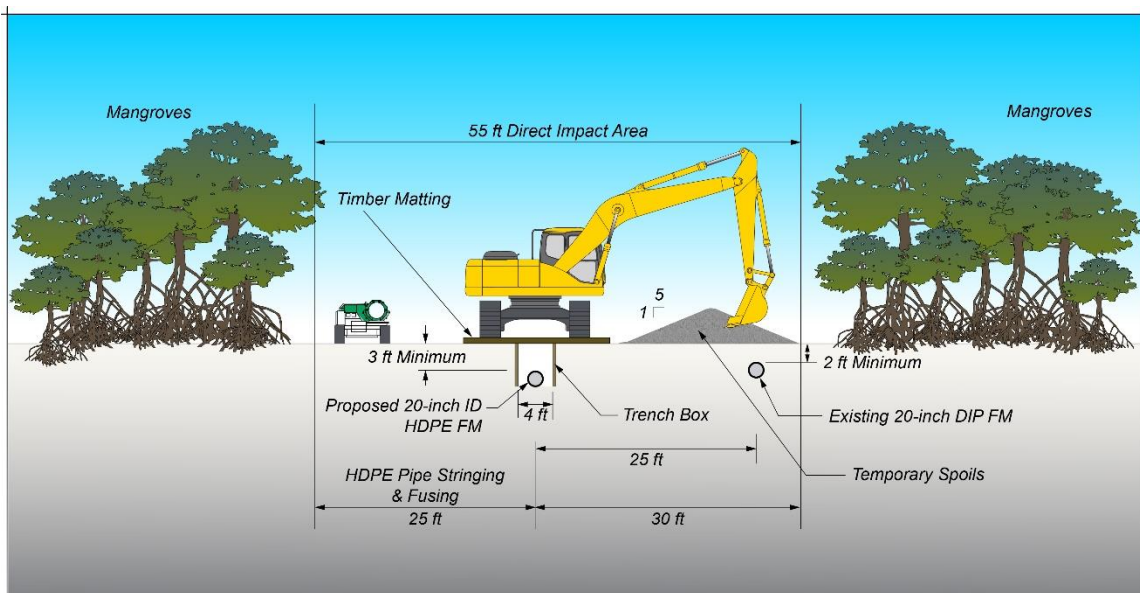
Figure 3-16 Typical Construction Section East Intertidal Zone (Segment 5)
