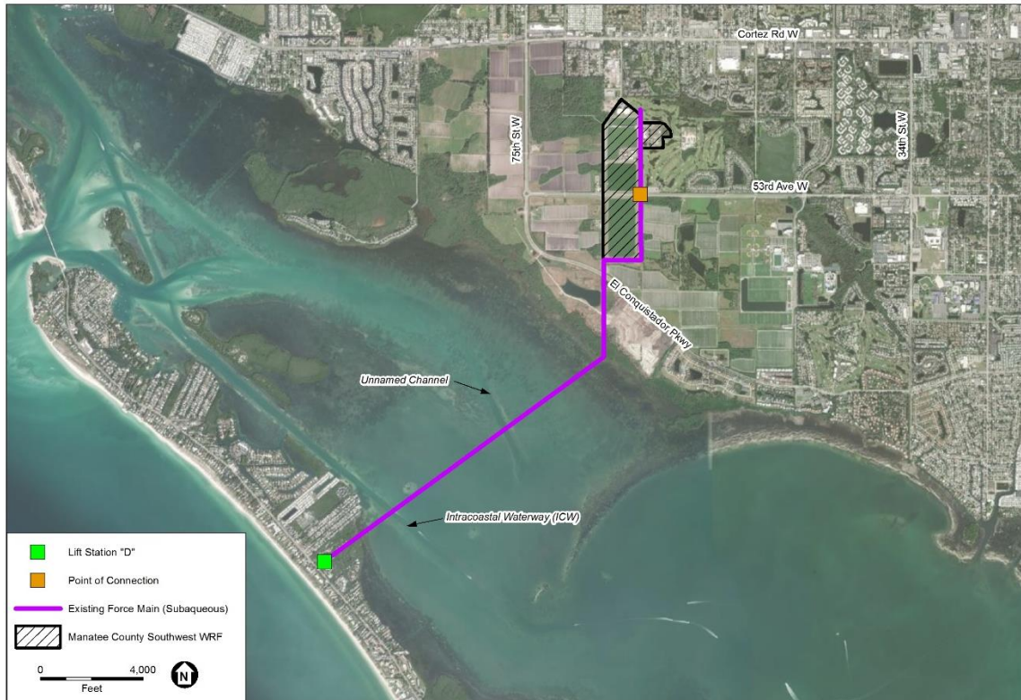
Figure 1-2 Existing Force Main Alignment
