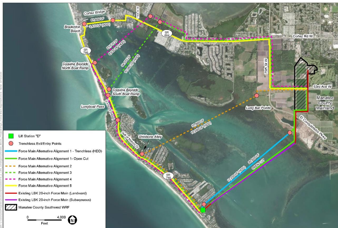
Figure 2-1 Force Main Alignment Alternatives
