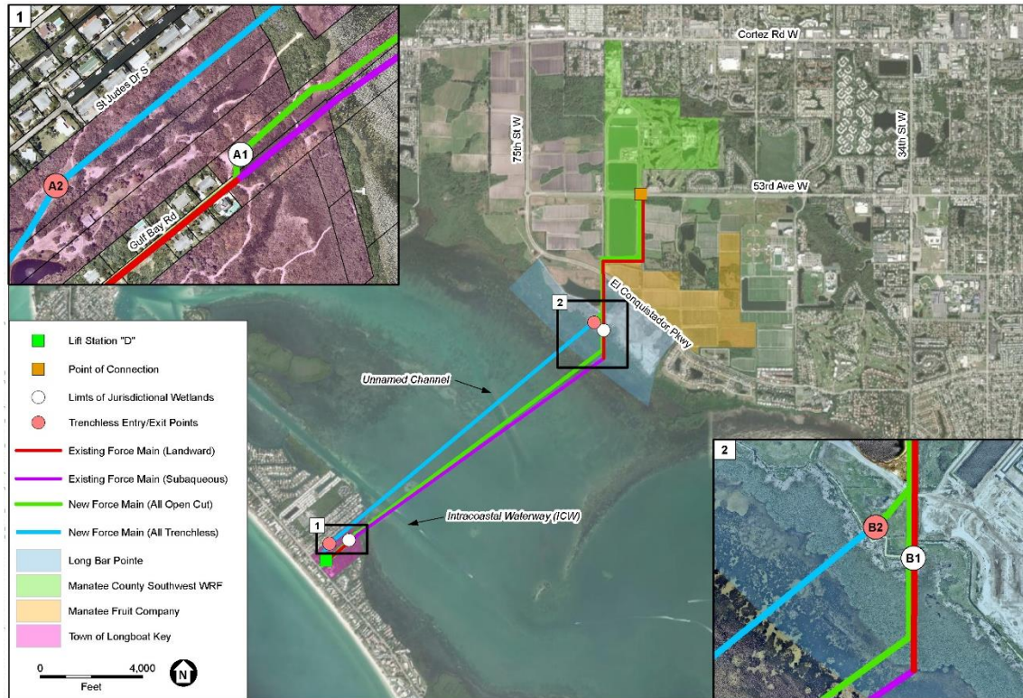
Figure 2-2 Plan View of Alignment 1
