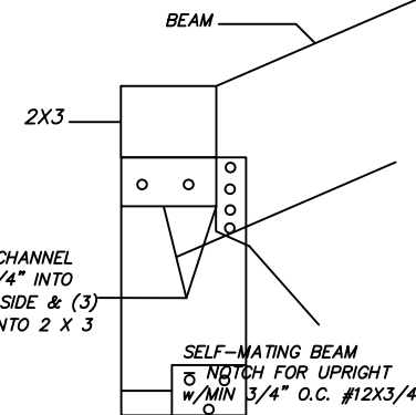
UPRIGHT TO BEAM CONNECTION DETAIL SCALE N.T.S.
