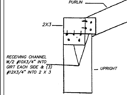
SLOPED PURLIN CONNECTION DETAIL SCALE N.T.S.
