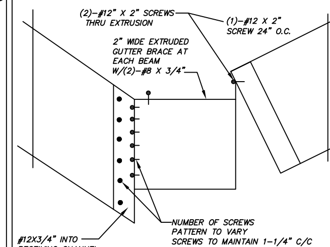
GUTTER BRACE & ANGLED FASCIA BOARD ATTACHMENT DETAIL SCALE N.T.S.
