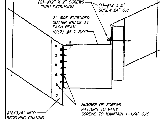
GUTTER BRACE & MATING ELEMENT ATTACHMENT DETAIL SCALE N.T.S.
