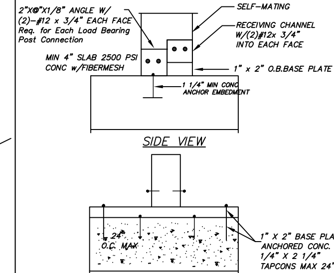
2" X 4" OR LARGER UPRIGHT TO DECK DETAILS SCALE N.T.S.
