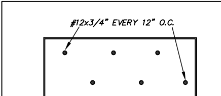
HEADER TO FACE OF GUTTER DETAIL SCALE N.T.S.
