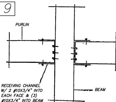
PURLIN OR GIRT TO BEAM OR POST DETAIL SCALE N.T.S.
