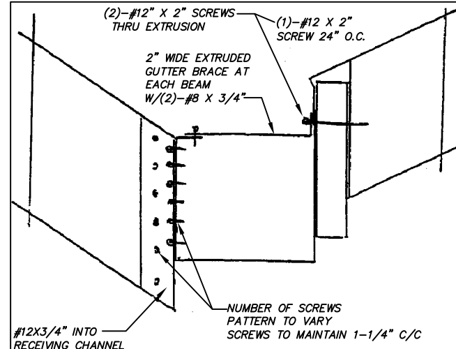
GUTTER BRACE & MATING ELEMENT ATTACHMENT DETAIL SCALE N.T.S.
