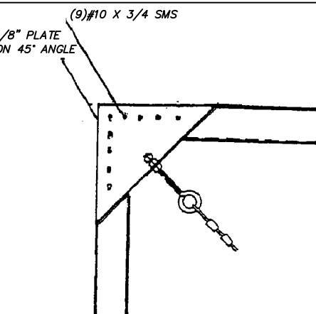
CABLE CONNECTION AT CORNER SCALE N.T.S.
