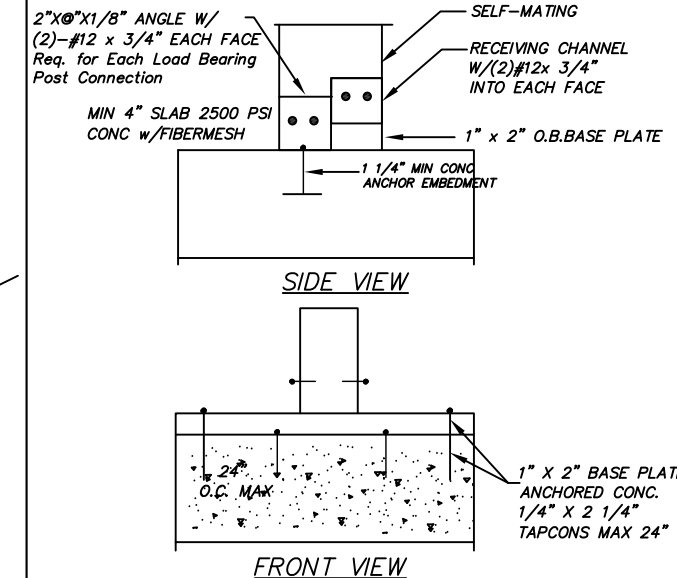
2" X 4" OR LARGER UPRIGHT TO DECK DETAILS SCALE N.T.S.
