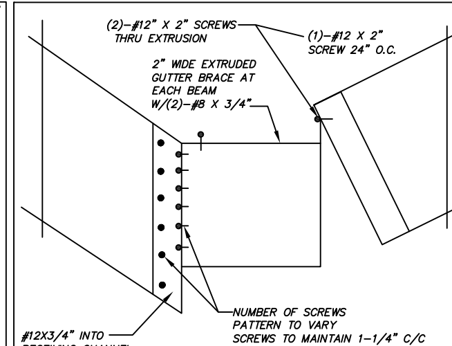
GUTTER BRACE & ANGLED FASCIA BOARD ATTACHMENT DETAIL SCALE N.T.S.
