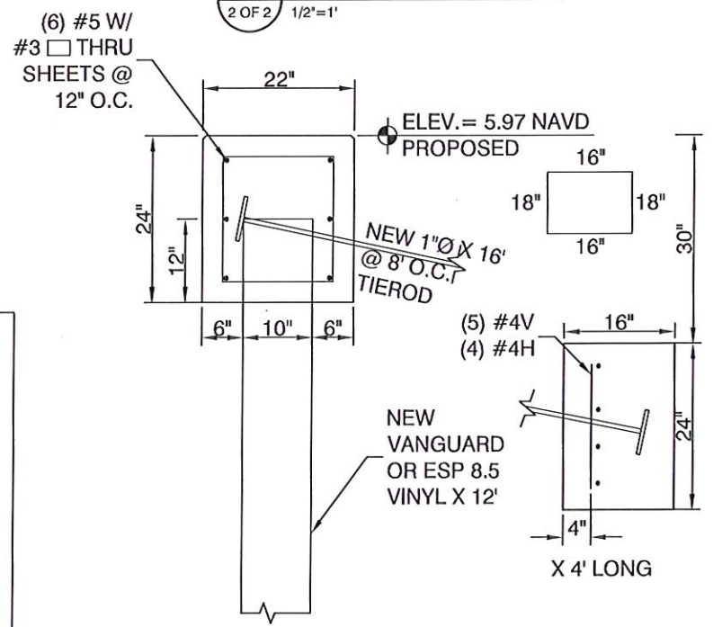
1 SEAWALL SECTION C VIEW - NEW 2 OF 2 1/2" = 1'
