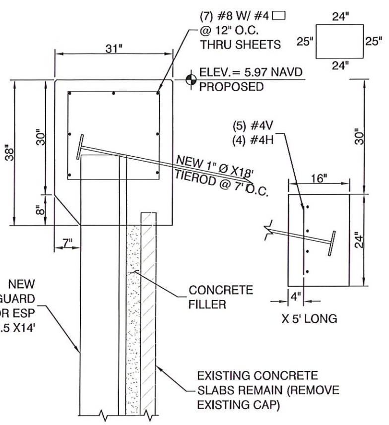
2 SEAWALL SECTION B VIEW 2 OF 2 1/2" = 1'
