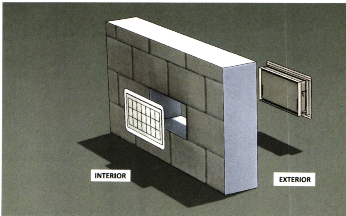
FIGURE 4—FLOOD VENT SEALING KIT
